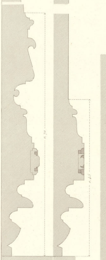
Base C. Fig. 4.
