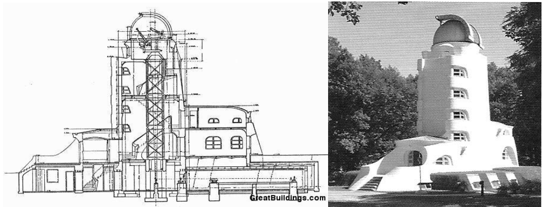
Şekil 4.49 E. Mendelsohn, Einstein Kulesi, Potsdam, Almanya, 1917-1921. ( www.greatbuildings.com ), (Yurttaş, 2009)
