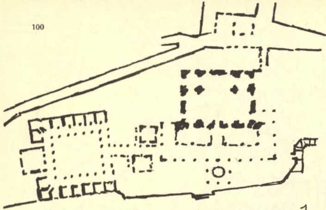
MİHRİMAH SULTAN CAMİİ PLANI 1547 - 48 İSTANBUL, ÜSKÜDAR MIHRIMAH SULTAN MOSQUE – ISTANBUL, ÜSKÜDAR 1547 - 48
