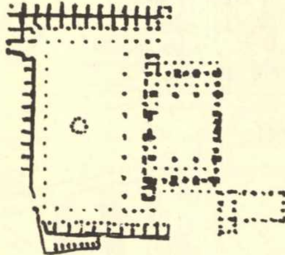
MİHRİMAH SULTAN CAMİİ PLAN 1540 İSTANBUL, EDİRNEKAPI MIHRIMAH SULTAN MOSQUE – PLAN 1540 ISTANBUL, EDİRNEKAPI
