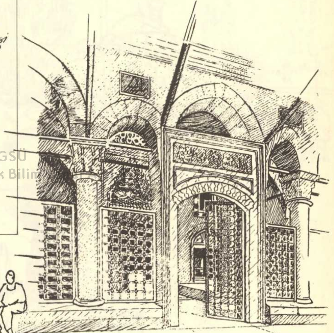
KILIÇ ALİ PAŞA CAMİİNDEN DETAY VE TÜRBE – İSTANBUL, TOPHANE DETAIL FROM KILIÇ ALİ PAŞA MOSQUE AND TOMB – ISTANBUL, TOPHANE
